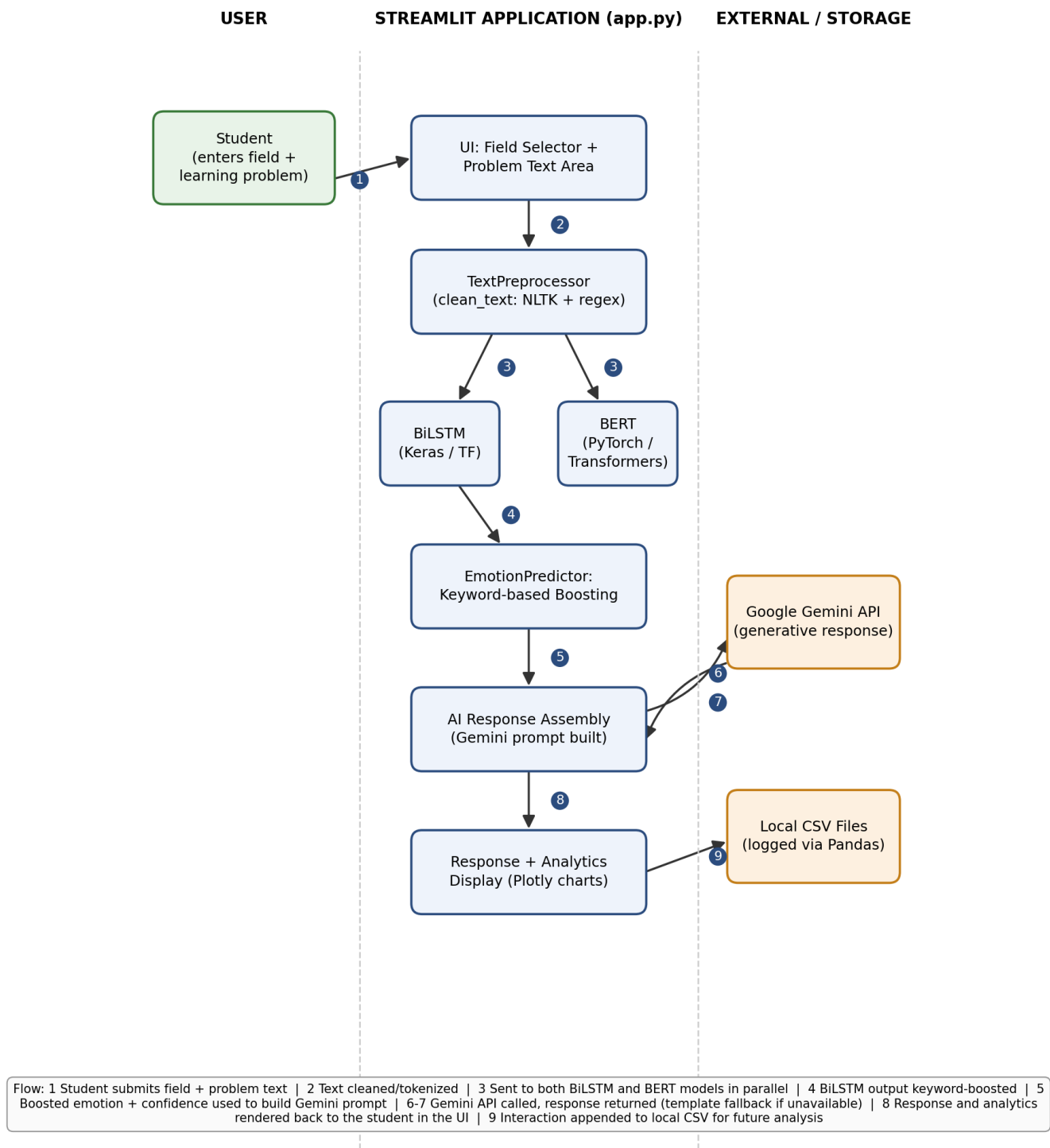
Figure 1: Architecture and data flow of the Emotion Detection and Learning Support Engine, showing how a student's text input flows through preprocessing, dual-model emotion classification (BiLSTM and BERT), keyword-based boosting, Gemini-powered response generation, and interaction logging.
